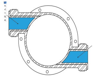
The new dual discharge port connection allow any pipework routing
